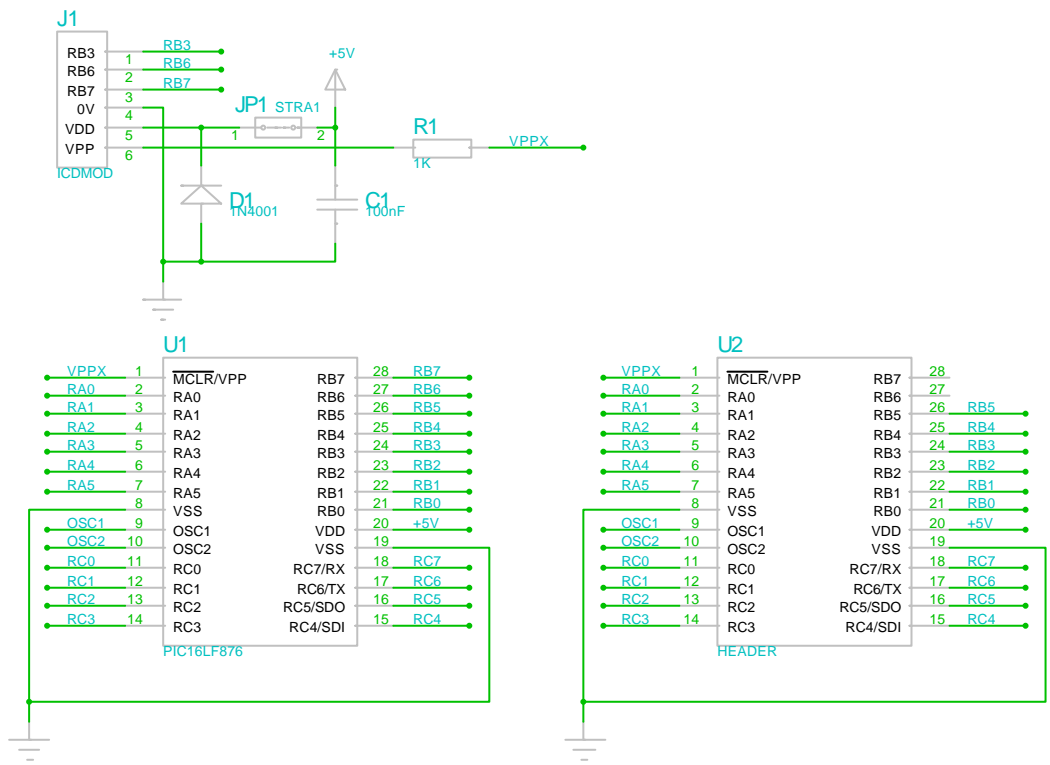
Header PIC16F876
